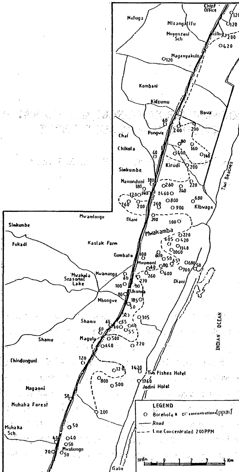
Figure 5.1 Concentration of chloride in boreholes in Diani-Tiwi area
